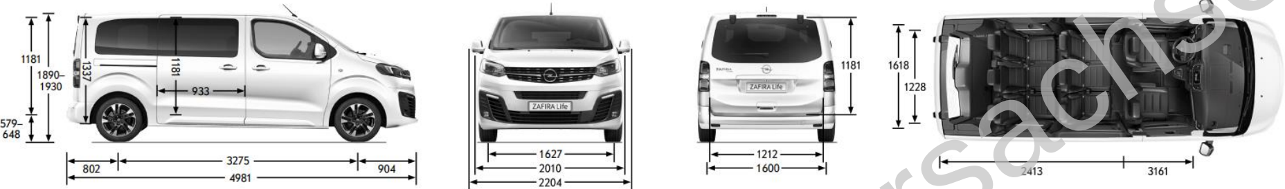
Zafira Electric Alle Maße in mm
